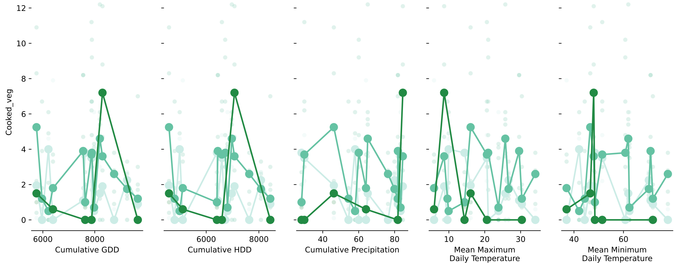
Under Ripe Ripe Over Ripe Climate impacts on Cooked_veg for Marquette, 2019
